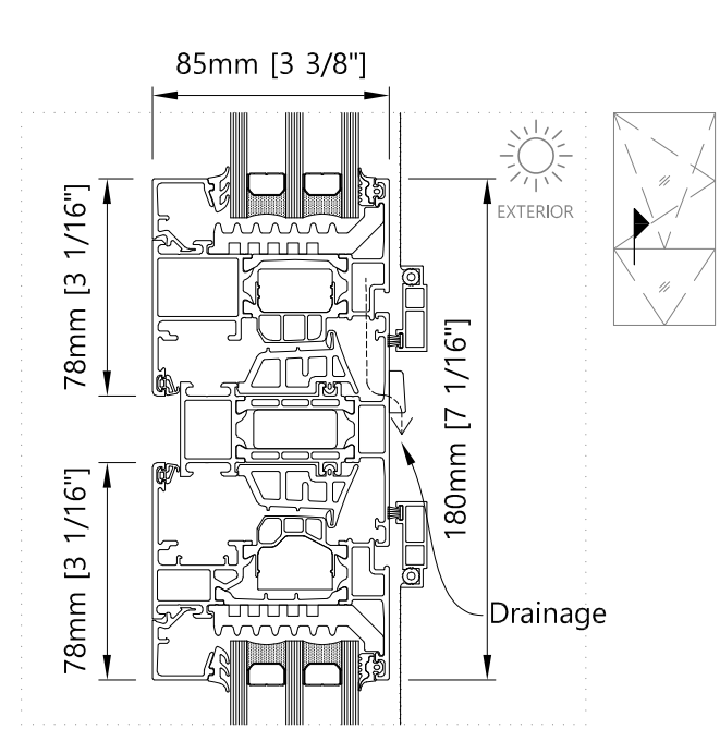
17 Transom - Vertical Motorized hopper window
