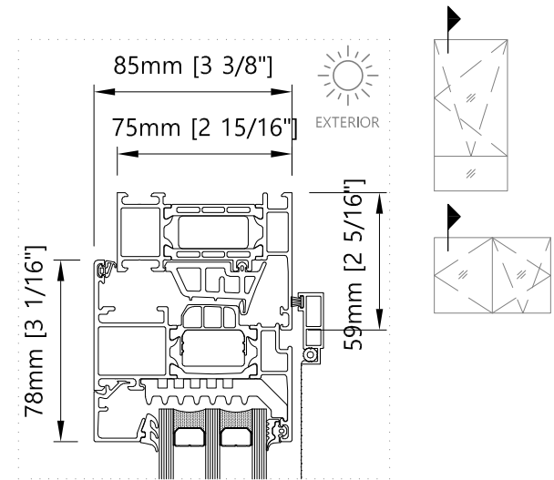
8 Top - Vertical T&T Window / Double T&T
